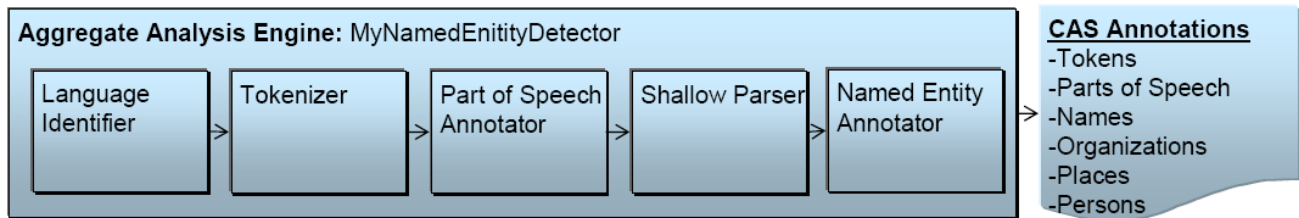
Figure 3. Sample Aggregate Analysis Engine
