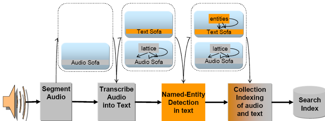
Figure 6. Multiple Sofas in support of multi-modal analysis of an audio Stream. Some engines work on the audio “view”, some on the text “view” and some on both.
