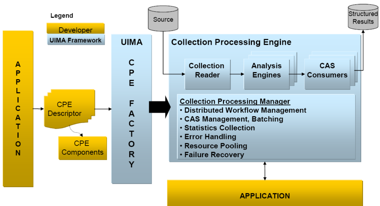
Figure 5. Collection Processing Manager in UIMA Framework
