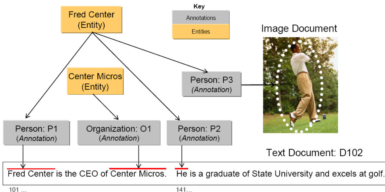
Figure 2. Objects represented in the Common Analysis Structure (CAS)
