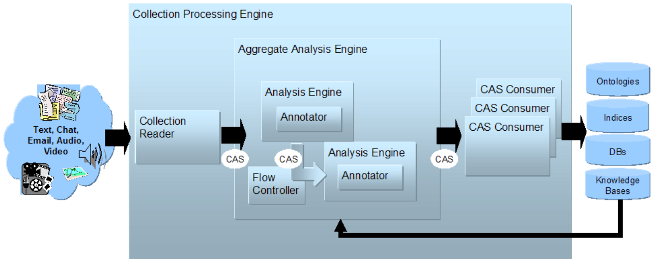
Figure 4. High-Level UIMA Component Architecture from Source to Sink
