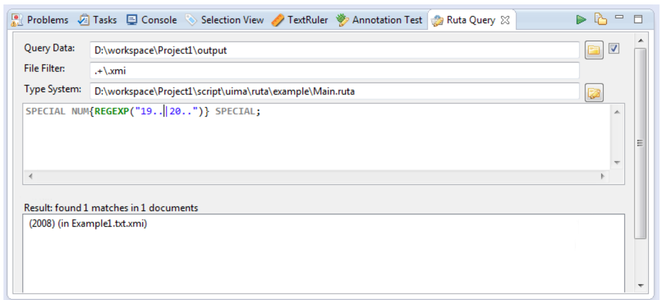
Figure 10. The Query View. *(1)*Start Button; *(2)*Export Button
