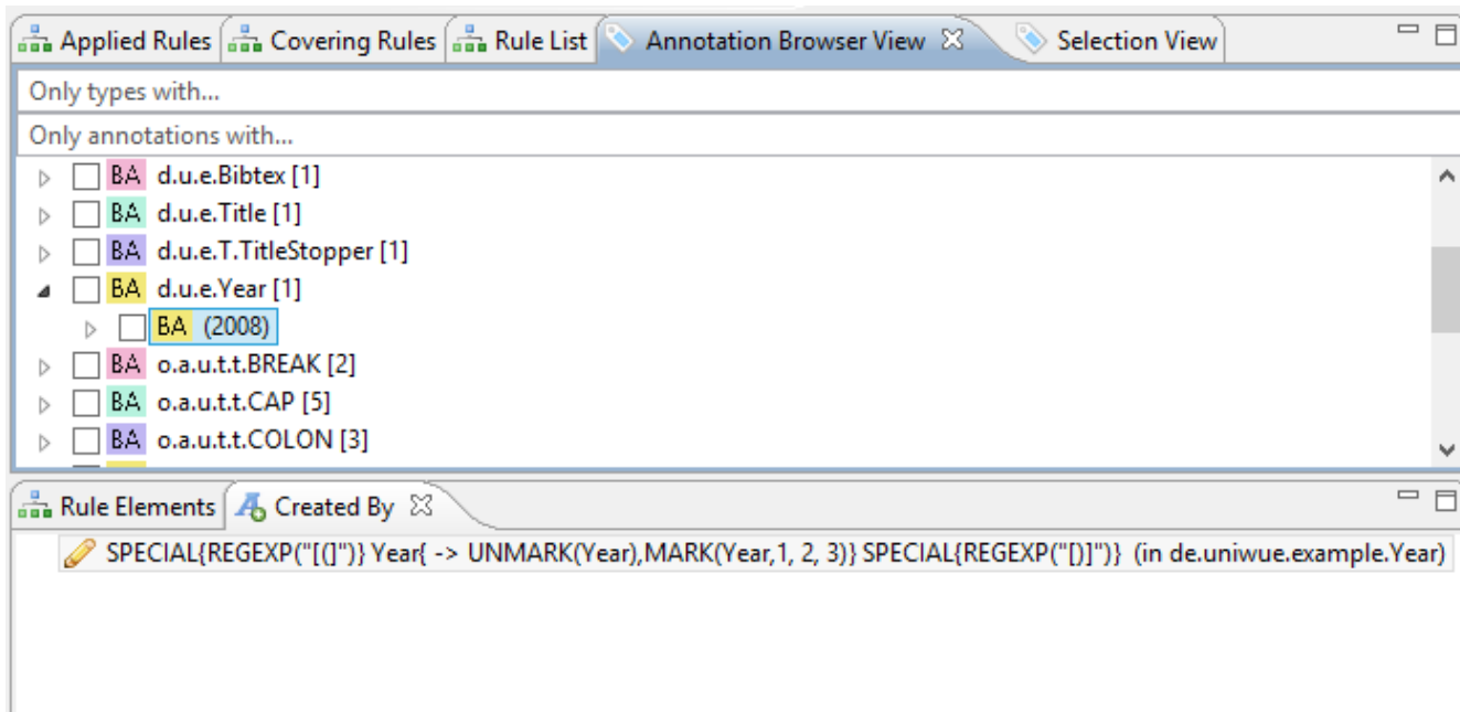
Figure 8. The Created By view
