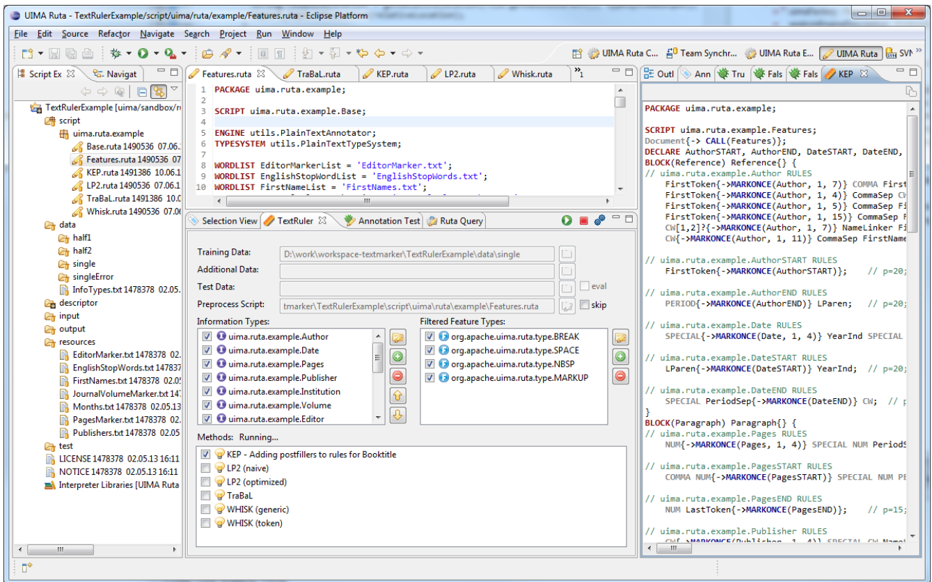
Figure 17. The UIMA Ruta TextRuler framework
