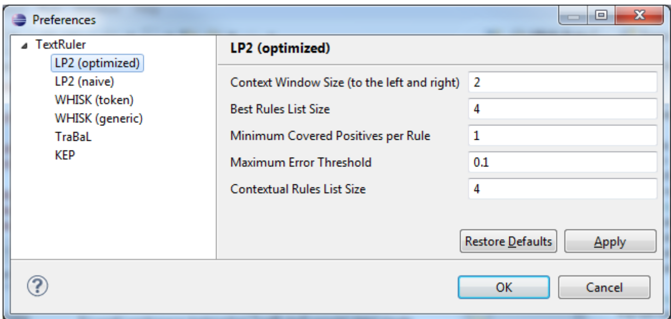
Figure 18. The UIMA Ruta TextRuler Preferences
