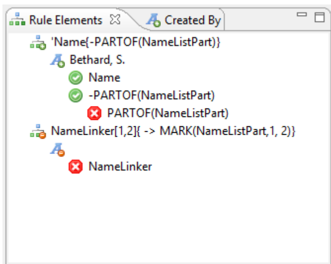
Figure 7. The views Matched Rules and Failed Rules
