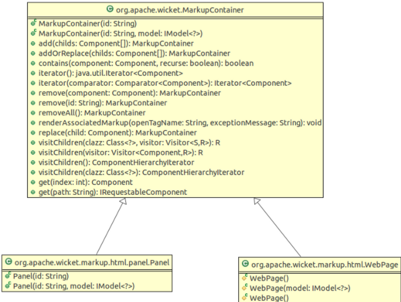
Illustration: Hierarchy of WebPage and Panel classes
